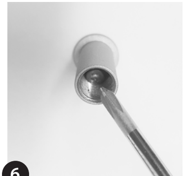
Mount Suspension Kit Body on to the ceiling.
